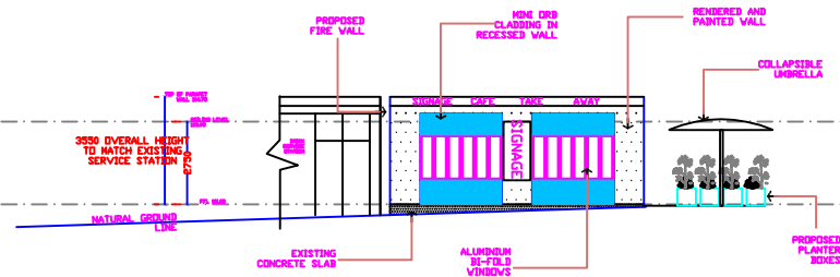
FRONT ELEVATION
