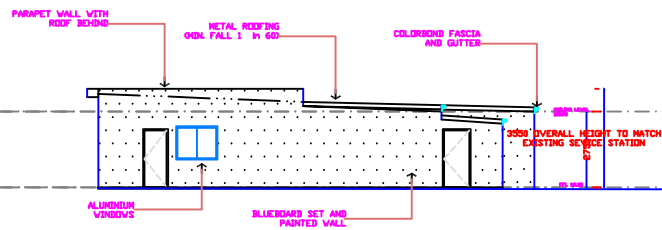
SIDE ELEVATION
